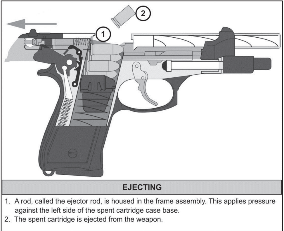
Figure 2-10. Ejecting example
