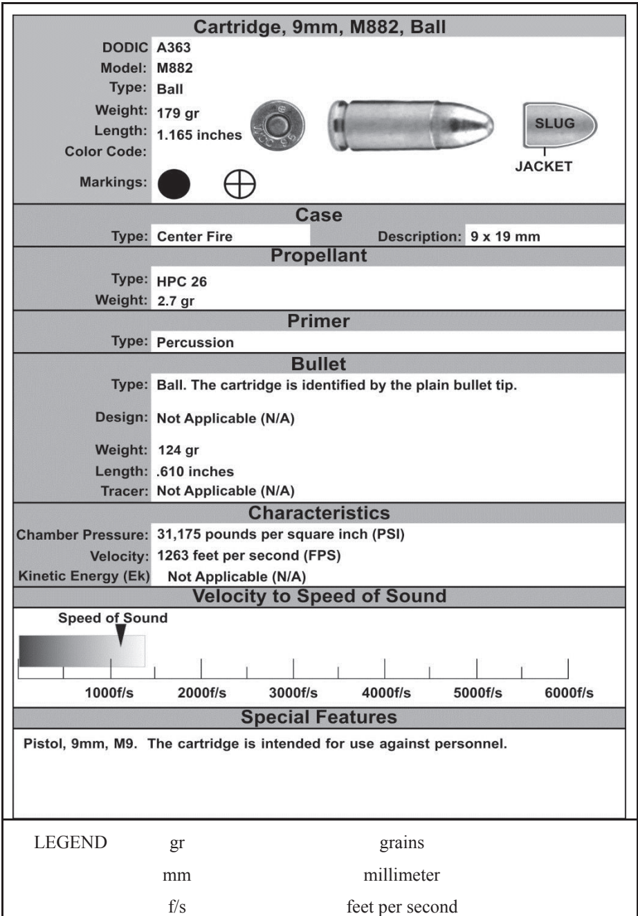
Figure A-1. M882 ball round
