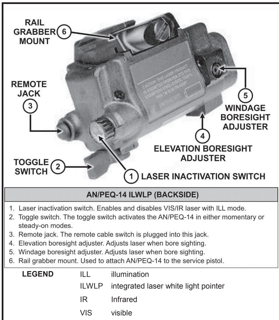
Figure 3-3b. AN/PEQ-14 operator controls (back)
