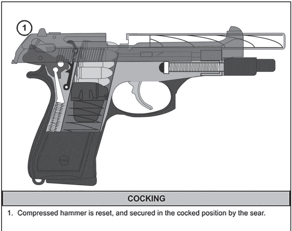
Figure 2-11. Cocking example
