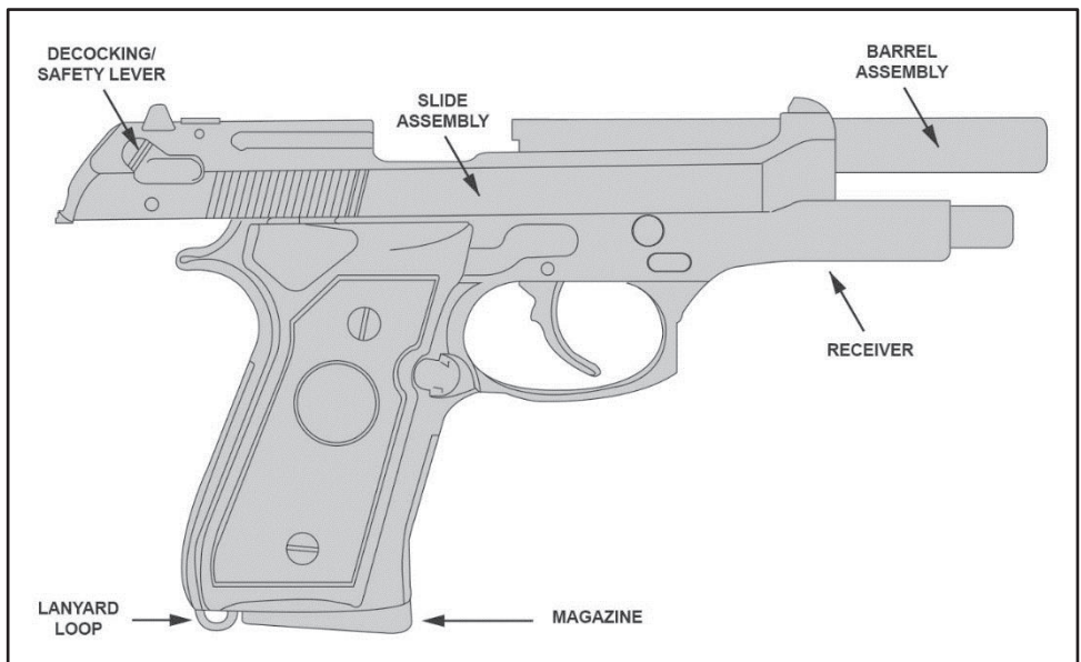
Figure 2-1. M9 service pistol
