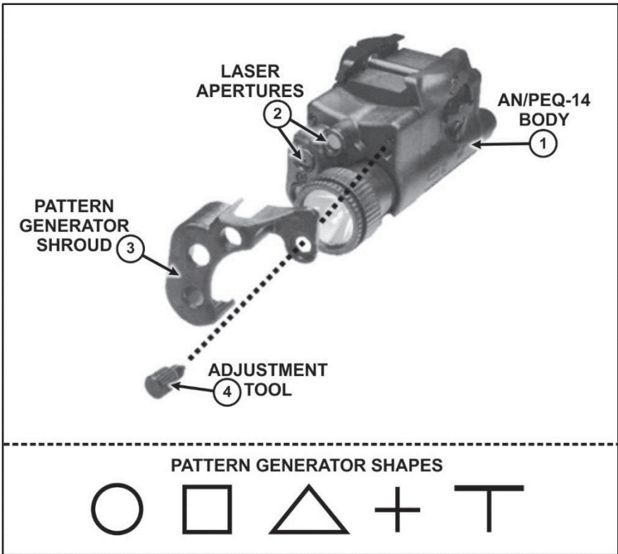
Figure 3-5. Pattern generator install
