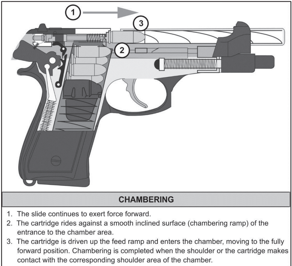
Figure 2-5. Chambering example
