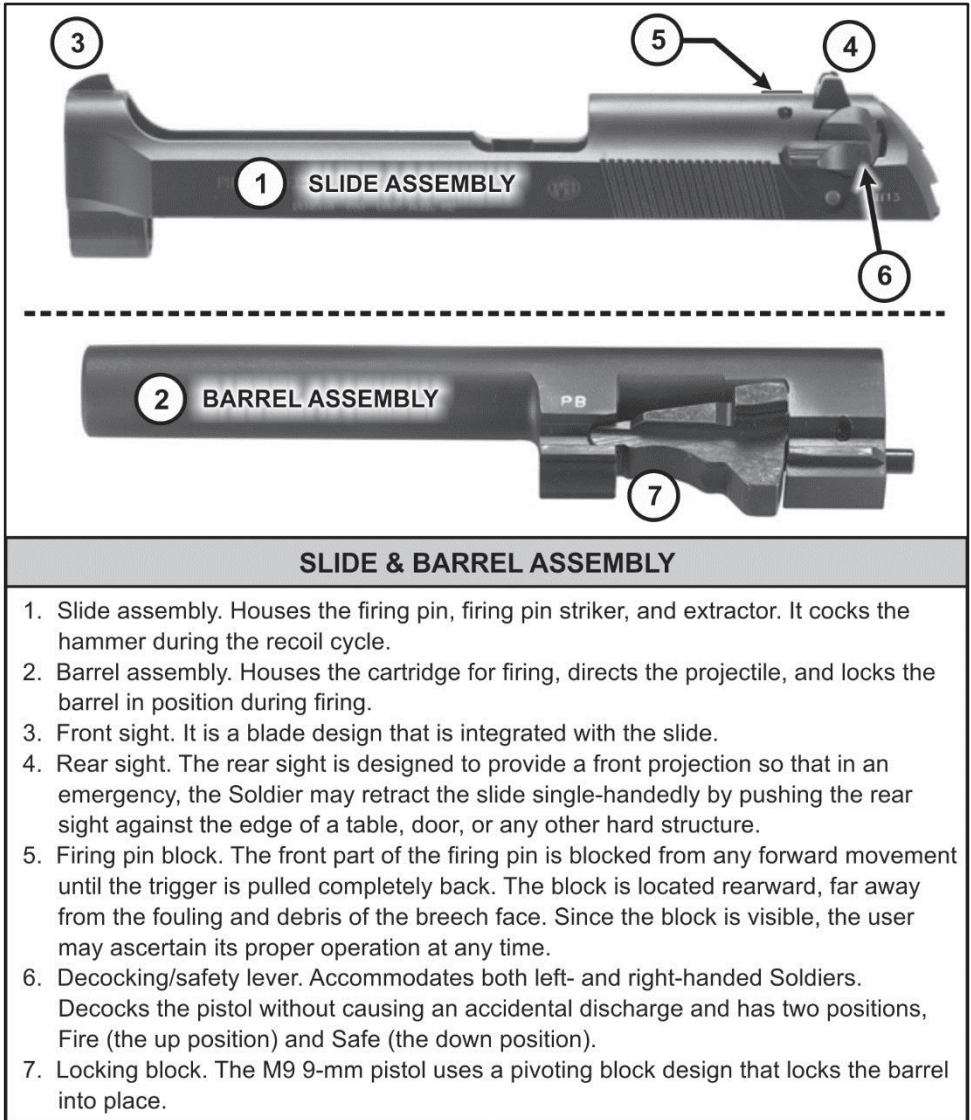
Figure 2-2. Slide and barrel assembly
