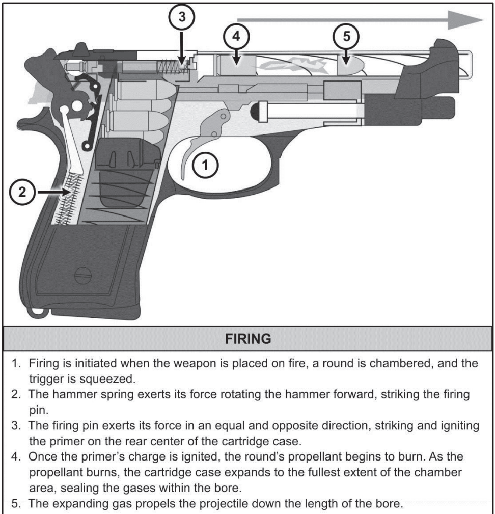
Figure 2-7. Firing example
