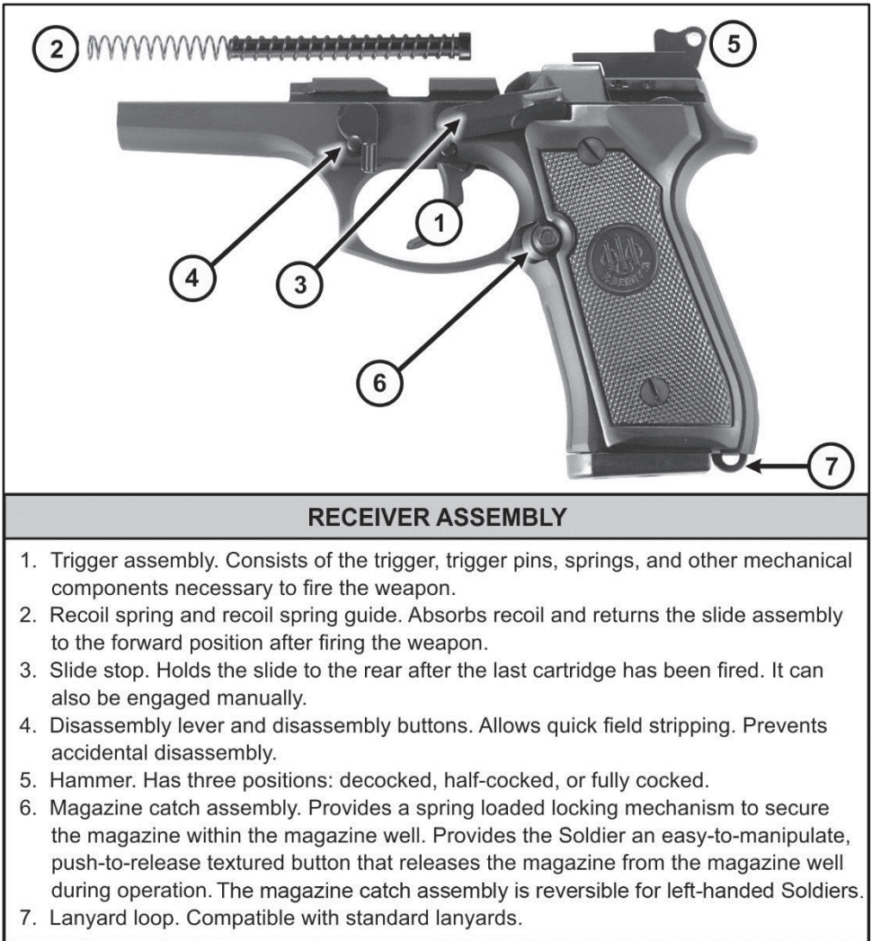
Figure 2-3. Receiver assembly
