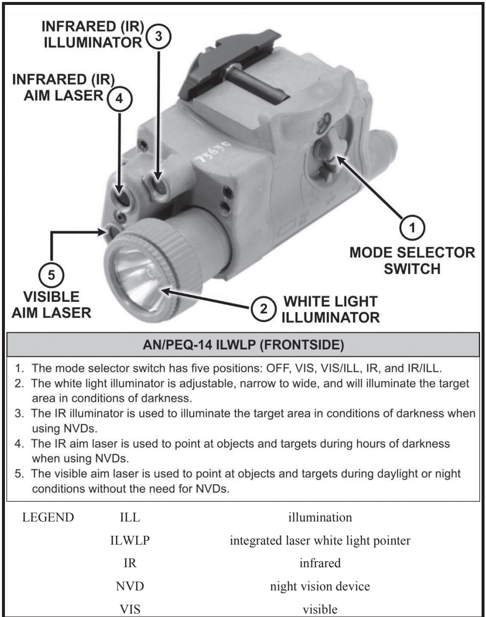
Figure 3-3a. AN/PEQ-14 operator controls (front)
