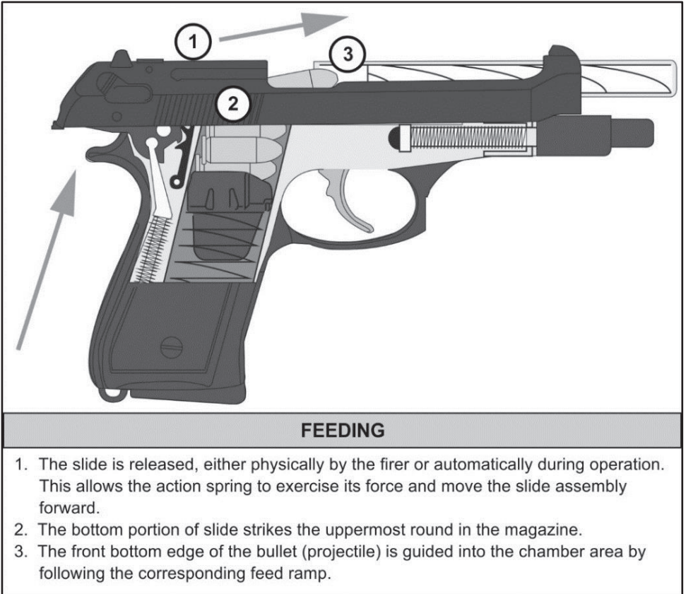
Figure 2-4. Feeding example
