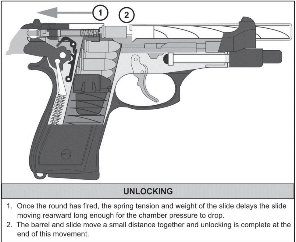
Figure 2-8. Unlocking example
