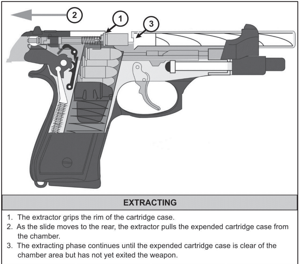
Figure 2-9. Extracting example
