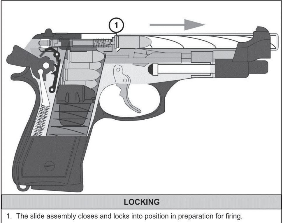
Figure 2-6. Locking example
